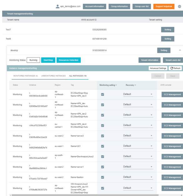
SIOS AppKeeper shows you the health status of all of your instances at a glance. You choose the response actions.
